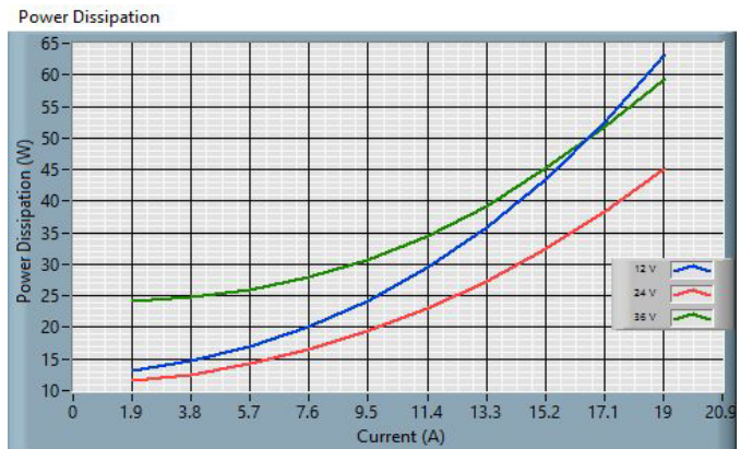
Fig. 16: 24S53.19FXW (ROHS) Power Dissipation
