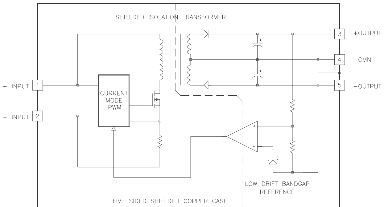
10 Watt Dual WD Series Block Diagram
