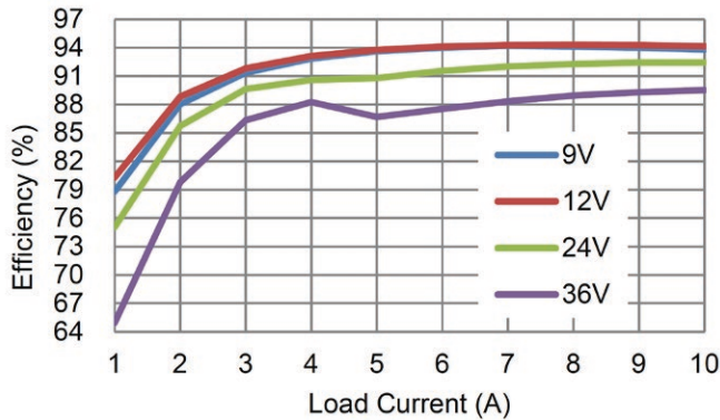
Fig. 12-1: Efficiency vs. Line and Load @ 25°C
