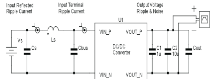
Fig. T1: Measurement Input Ripple and Output Noise Circuit
