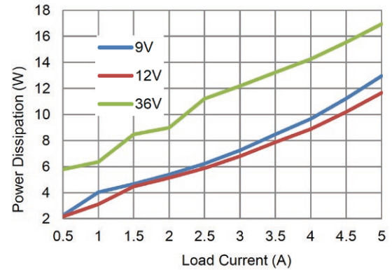
Fig. 24-2: Power Dissipation vs. Load @ 25°C
