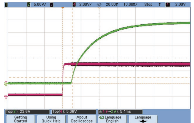
Fig. 24-6: Transient response, Vout = Nom, Iout = 50-75% Step
