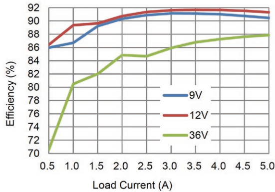
Fig. 24-1: Efficiency vs. Line and Load @ 25°C
