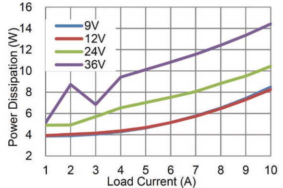
Fig. 12-2: Power Dissipation vs. Load @ 25°C
