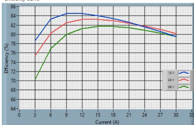
Efficiency Curve
