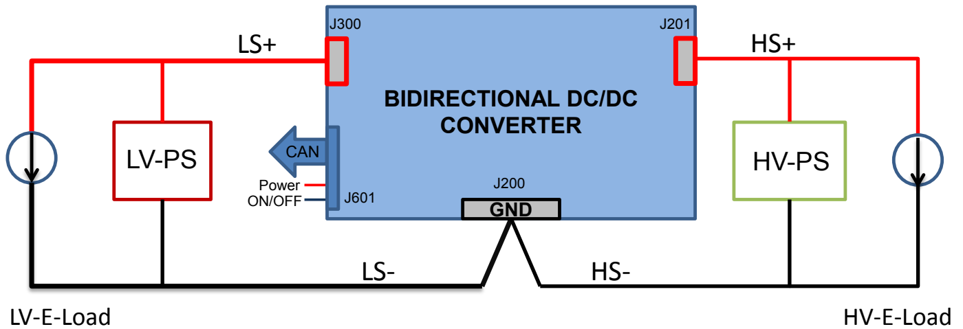
Fig. 2: The bench setup used to operate 48S12.3K0BCA and take measurements provided in data sheet. The combination of the Electronic Load (E-Load) and Bench Power Supply (PS) emulates a battery capable of both sourcing and sinking current.
