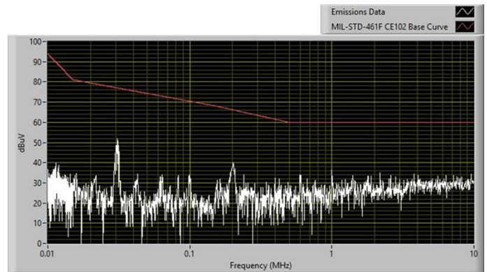
b) With input filter from Fig. 28.
