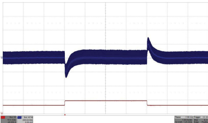
Fig. 30: Output voltage response to load current step change 50% - 75% - 50% (6.5A – 9.75A – 6.5A) with di/dt = 1A/μs at VIN = 24V. Top trace (C4): Output voltage (200 mV/div.). Bottom trace (C3): Load current (10A/div.). C o 470μF/70mΩ. Time: 1ms/div.
