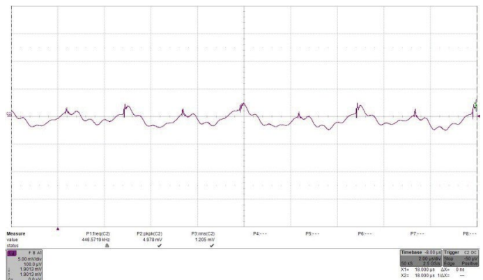
Fig. 27: Input reflected ripple current, i_C (500 mA/mV), measured at input terminals at full rated load current at VIN = 24V. Refer to Fig. 2 for test setup. Time: 2 \mu s/div. RMS input ripple current is 1.205 \times 500mA = 602.5mA .
