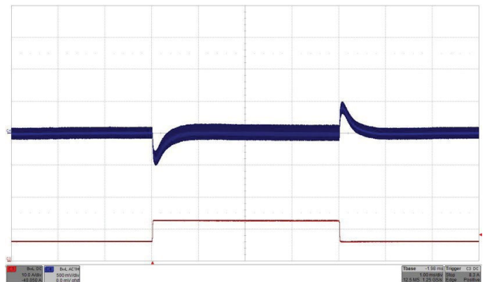
Fig. 31: Output voltage response to load current step change 50% - 100% - 50% (6.5A – 13A – 6.5A) with di/dt = 1A/μs at VIN = 24V. Top trace (C4): Output voltage (500 mV/div.). Bottom trace (C3): Load current (10A/div.). C o 470μF/70mΩ. Time: 1ms/div.
