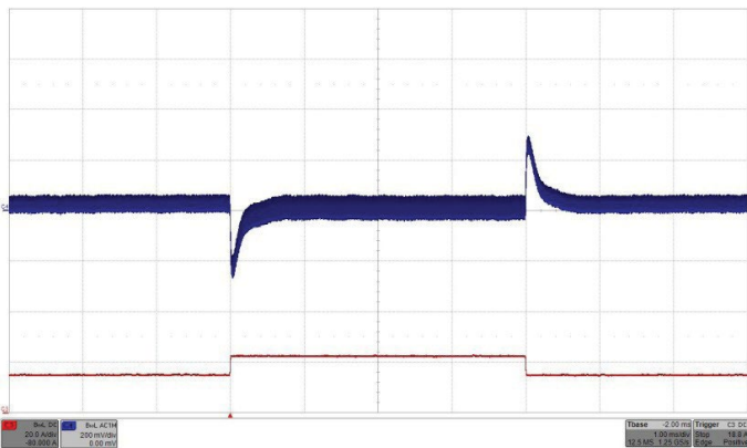
Fig. 18: Output voltage response to load current step change 50% - 75% - 50% (15A – 22.5A – 15A) with di/dt = 1A/μs at VIN = 24V. Top trace (C4): Output voltage (200 mV/div.). Bottom trace (C3): Load current (20A/div.). C o 470μF/70mΩ. Time: 1ms/div.
