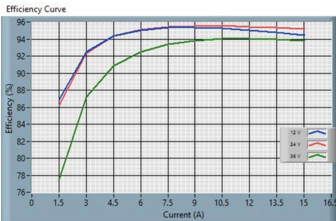
Fig. 6: 24S24.15MTW (ROHS) Efficiency Curve
