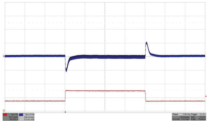
Fig. 19: Output voltage response to load current step change 50% - 100% - 50% (15A – 30A – 15A) with di/dt = 1A/μs at VIN = 24V. Top trace (C4): Output voltage (500 mV/div.). Bottom trace (C3): Load current (20A/div.). C o 470μF/70mΩ. Time: 1ms/div.
