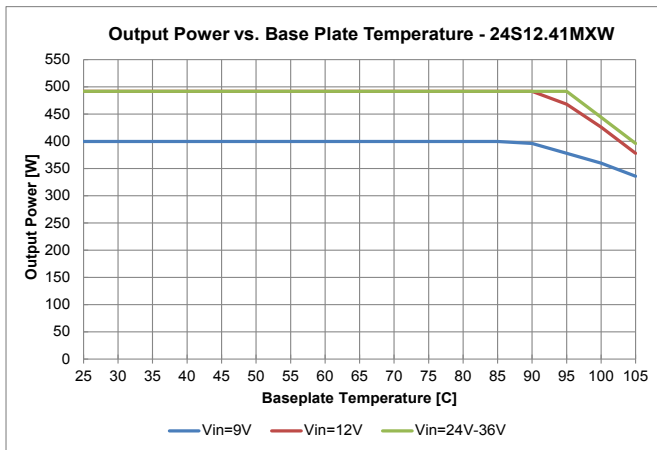
Fig. 10: 24S12.41MXW (ROHS) Derating Curve
