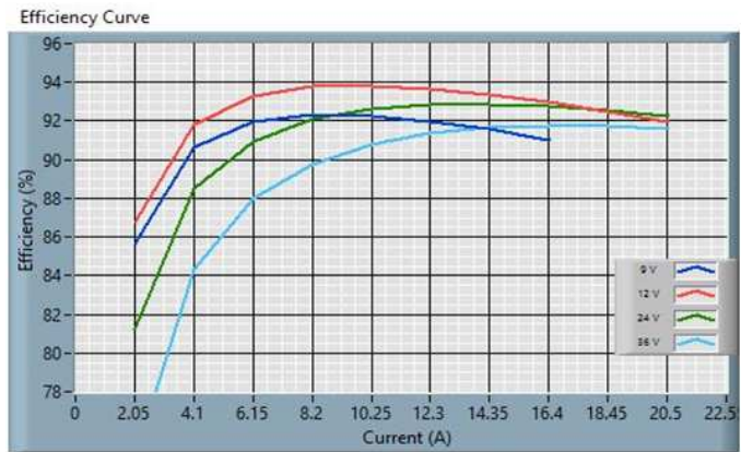
Fig. 4: Efficiency Curve
