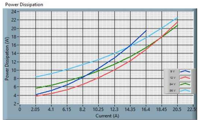
Fig. 5: Power Dissipation
