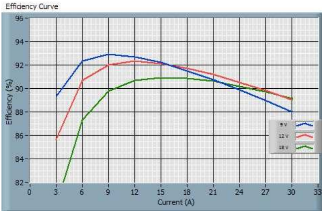
Fig 4-1: 12S3.30QRW Efficiency Curve
