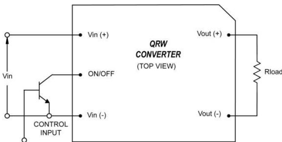
Fig 1: Circuit configuration for ON/OFF function.
