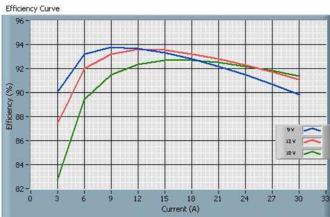
Fig 4-2 12S5.30QRW Efficiency Curve
