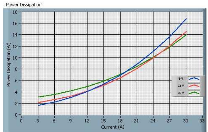
Fig. 5-2 12S5.30QRW Power Dissipation
