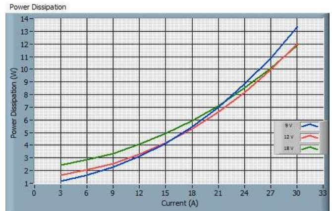
Fig 5-1: 12S3.30QRW Power Dissipation
