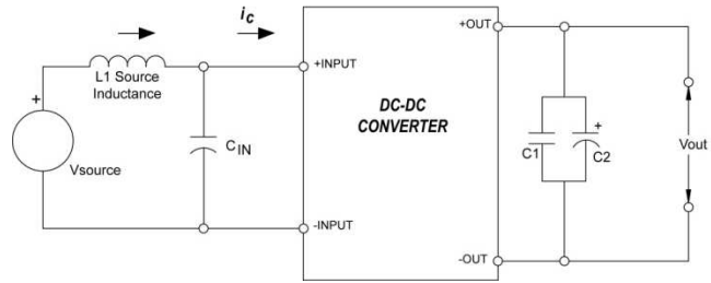
Fig. 2: Test setup for measuring input reflected ripple currents i_c
