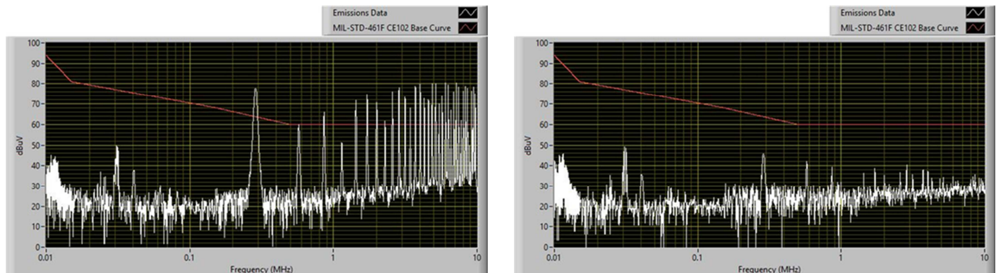
a) Without input filter. C9 = 330 \mu F/50V.
