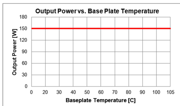
Figure A: Power derating as function of baseplate temperature
