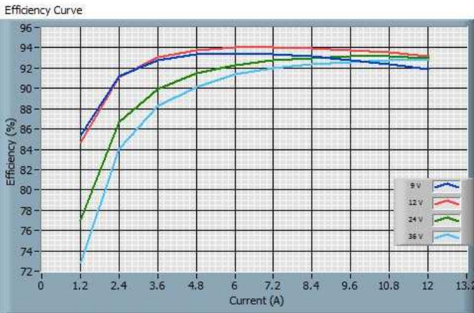
Fig. 4: 24S12.12QSW Efficiency Curve
