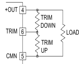
USING FIXED RESISTORS
