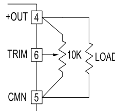
USING TRIM POT
