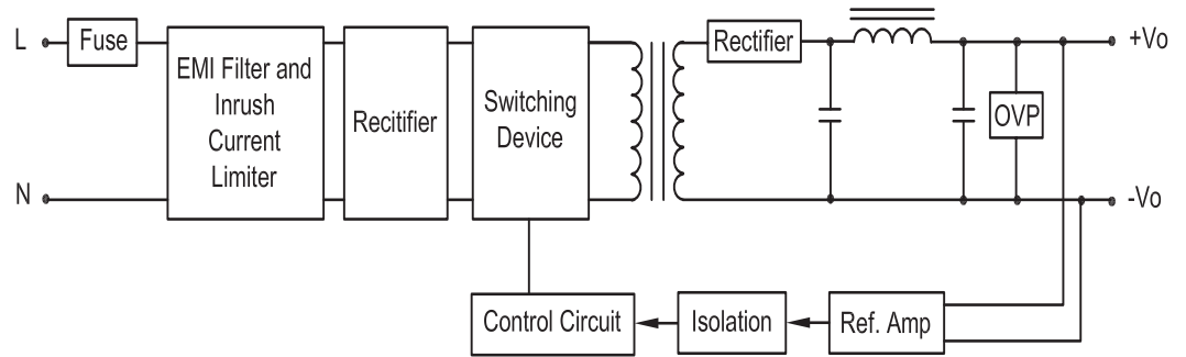
Single Output
